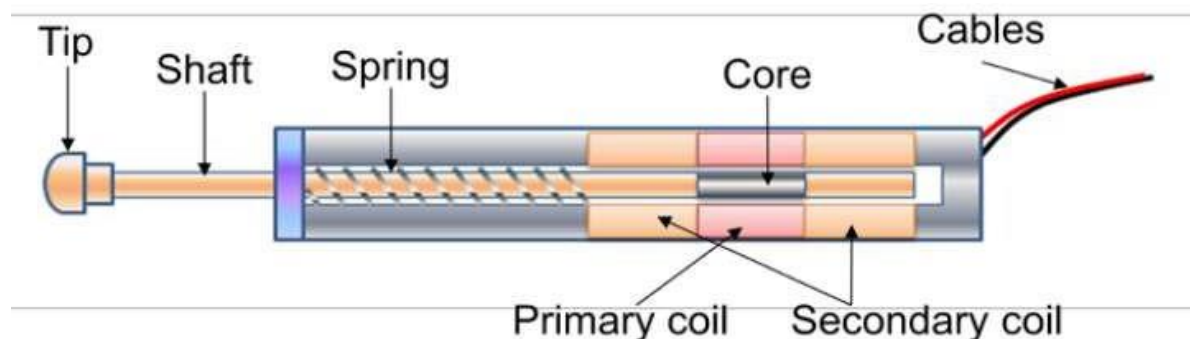
Construction of a LVDT sensor
