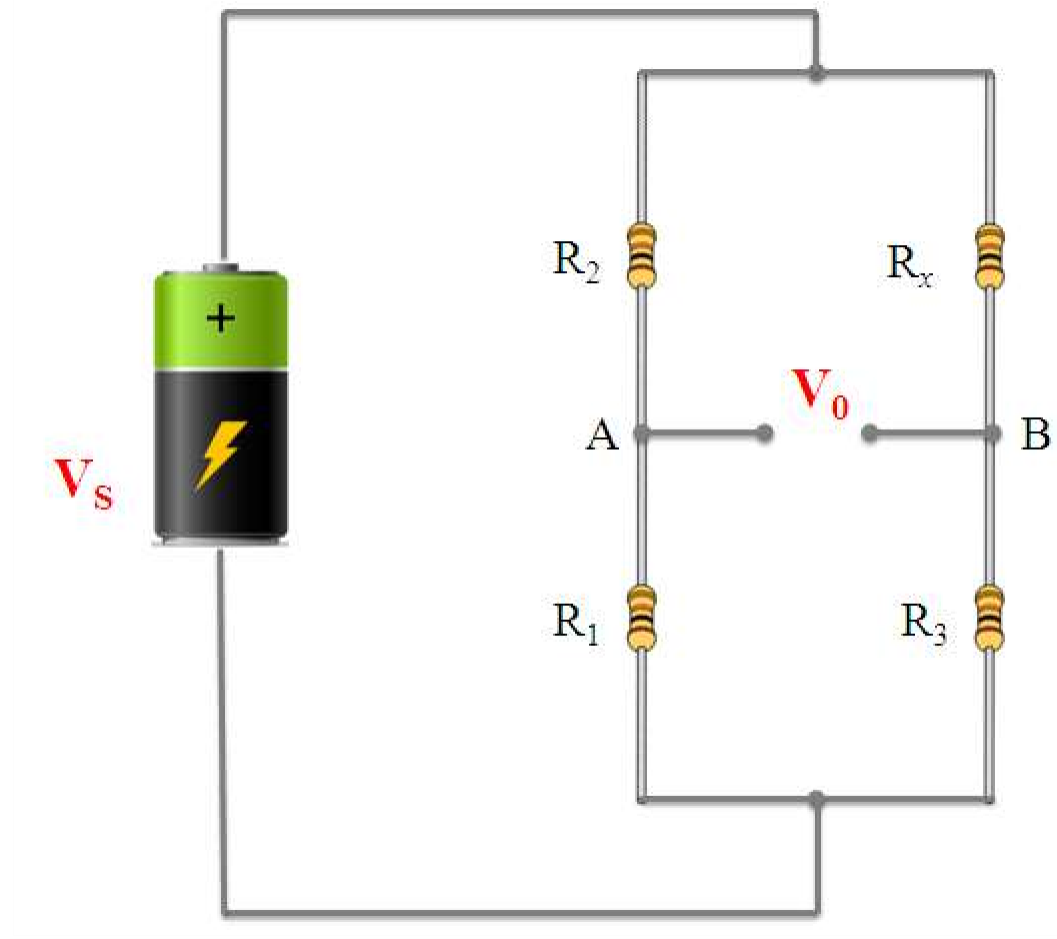
Wheatstone's bridge
