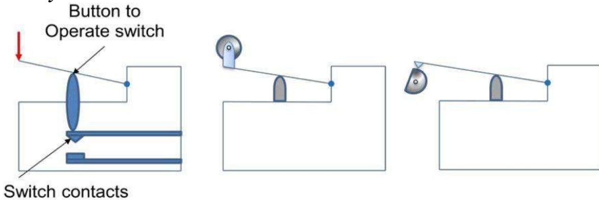
(a) Lever-operated
